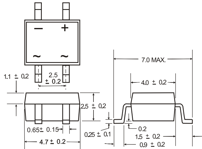
Dimensions in millimeters(1mm =0.0394英寸)
